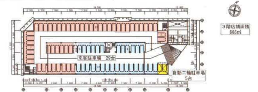
3階平面図 (3rd floor plan)
