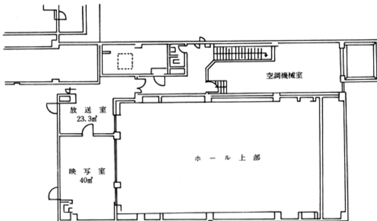
3 階 (166.95 m²)
